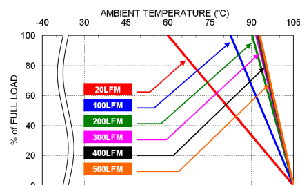
QAE60-72S05U Derating Curve With 0.5" Height Heat-sink (See Thermal Considerations)
